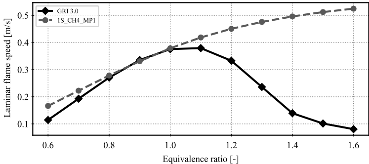
1D Premixed freely propagating flame at P = 1.0 bar and T = 300 K
