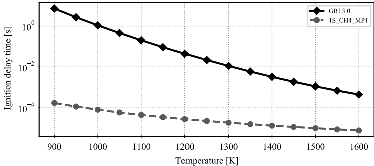
0D Isochoric reactor at P = 1.0 bar and phi = 1
